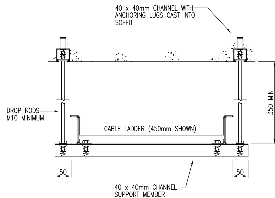
CABLE LADDER SUPPORT DETAIL (Not To Scale)
