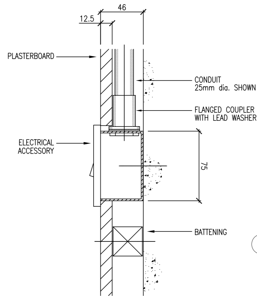
ACCESSORY INSTALLATION DETAIL (Not To Scale)
